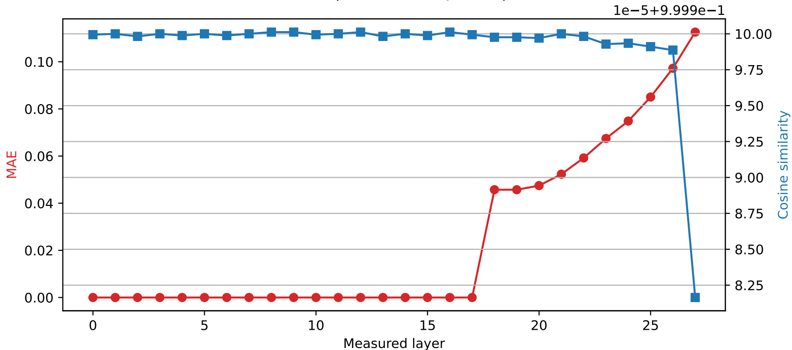
Qwen2.5-7B-Instruct | Quantized layer 17 | float32 \rightarrow int8
