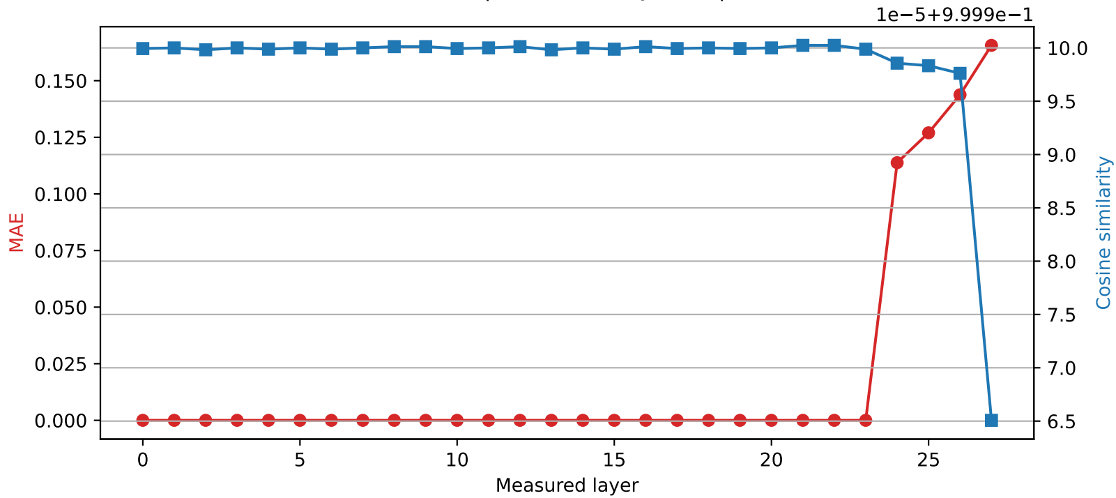
Qwen2.5-7B-Instruct | Quantized layer 23 | float32 \rightarrow int8
