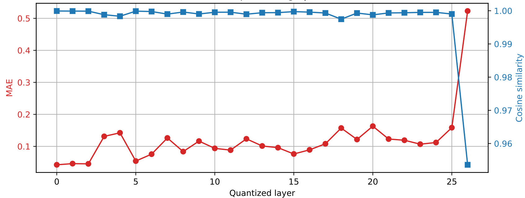
Qwen2.5-7B-Instruct | Prompt 3 Final RMSNorm output damage | float32 → int8
