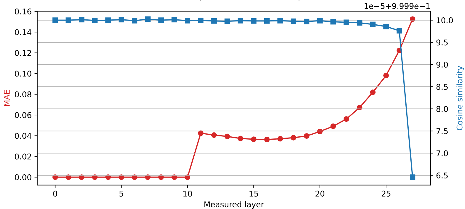
Qwen2.5-7B-Instruct | Quantized layer 10 | float32 \rightarrow int8
