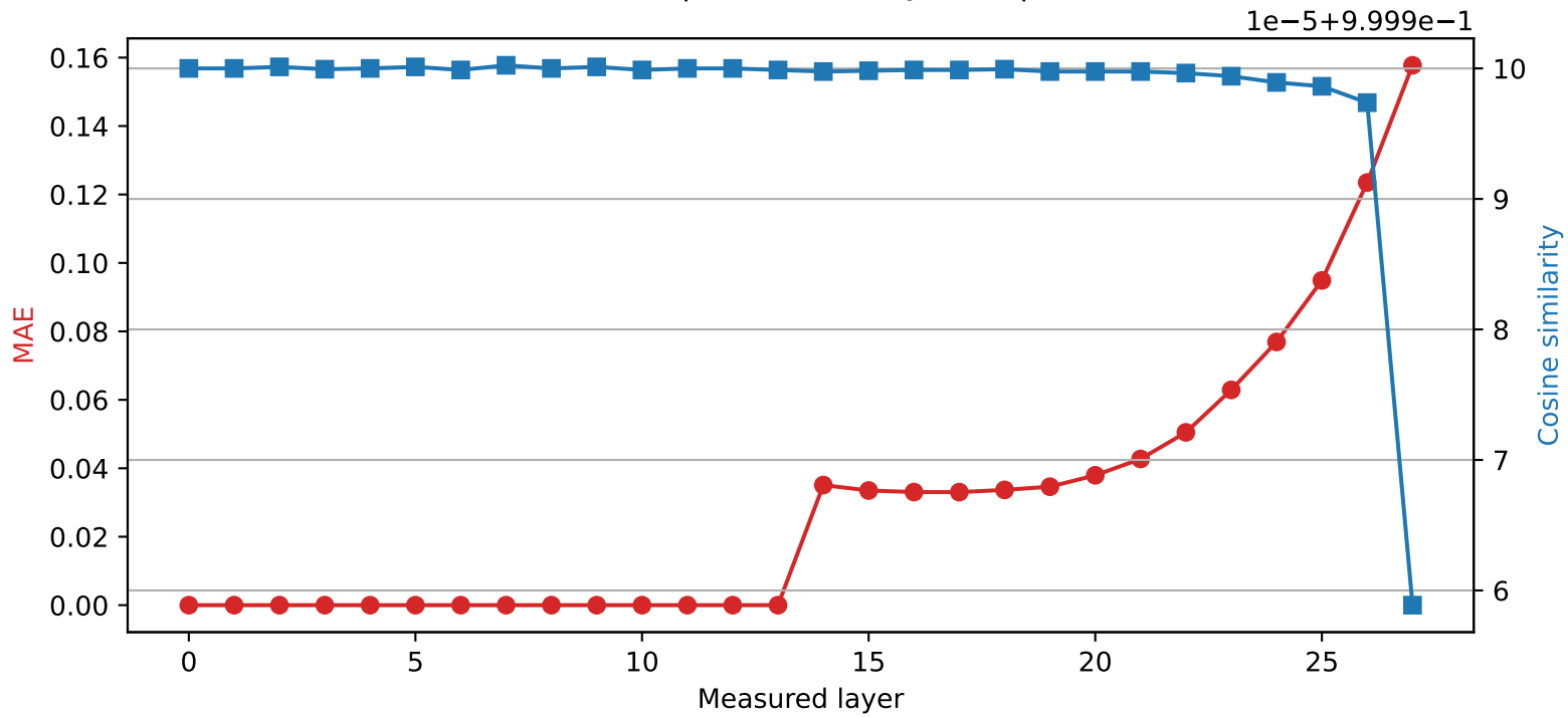
Qwen2.5-7B-Instruct | Quantized layer 13 | float32 \rightarrow int8
