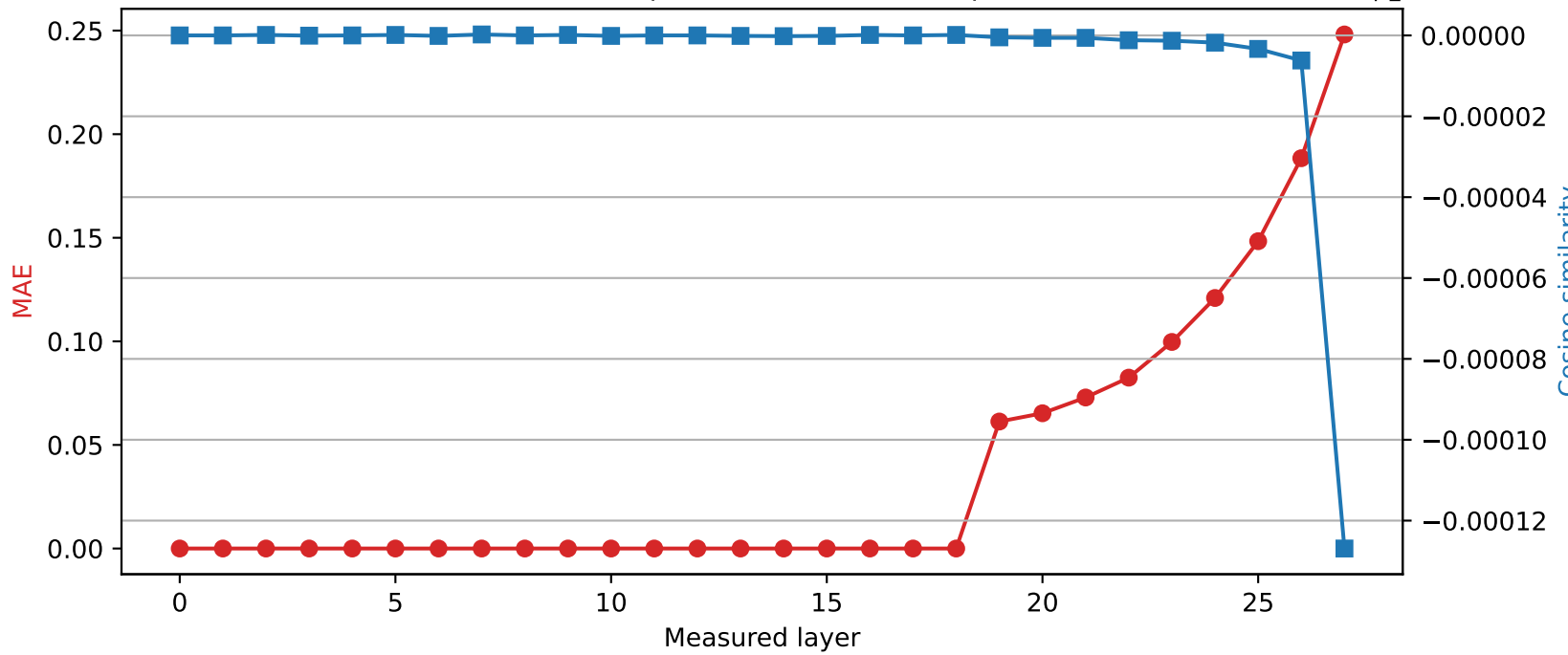
Qwen2.5-7B-Instruct | Quantized layer 18 | float32 \rightarrow int8
