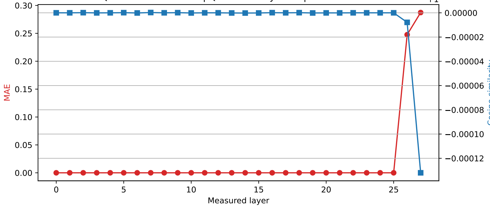
Qwen2.5-7B-Instruct | Quantized layer 25 | float32 → int8
