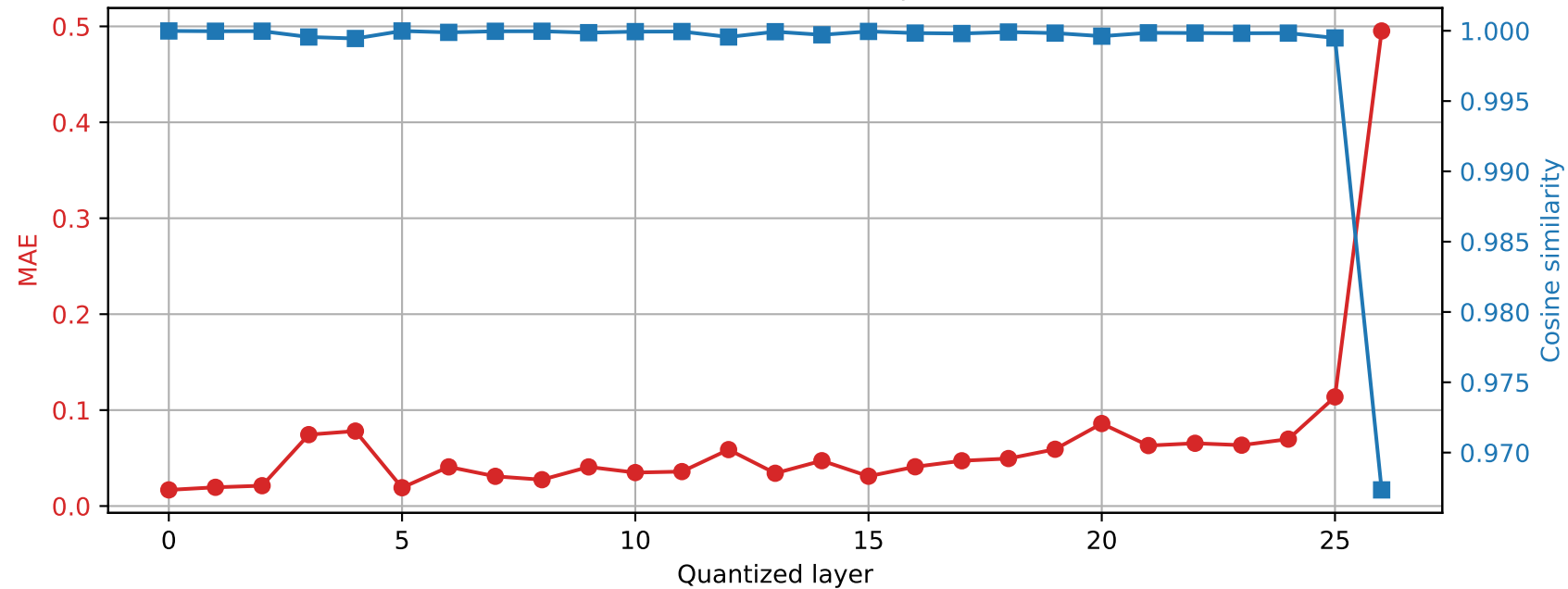
Qwen2.5-7B-Instruct | Prompt 4 Final RMSNorm output damage | float32 → int8
