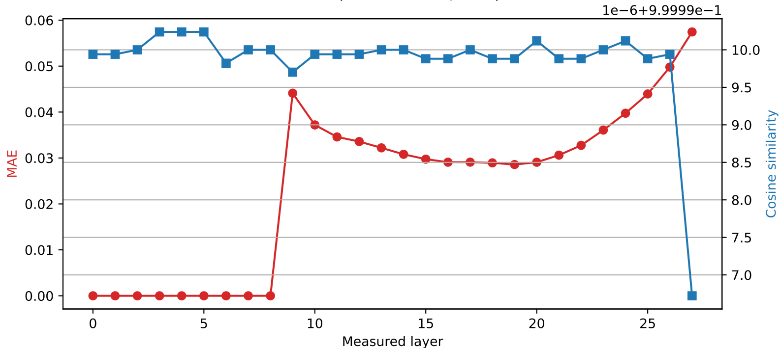
Qwen2.5-7B-Instruct | Quantized layer 8 | float32 → int8
