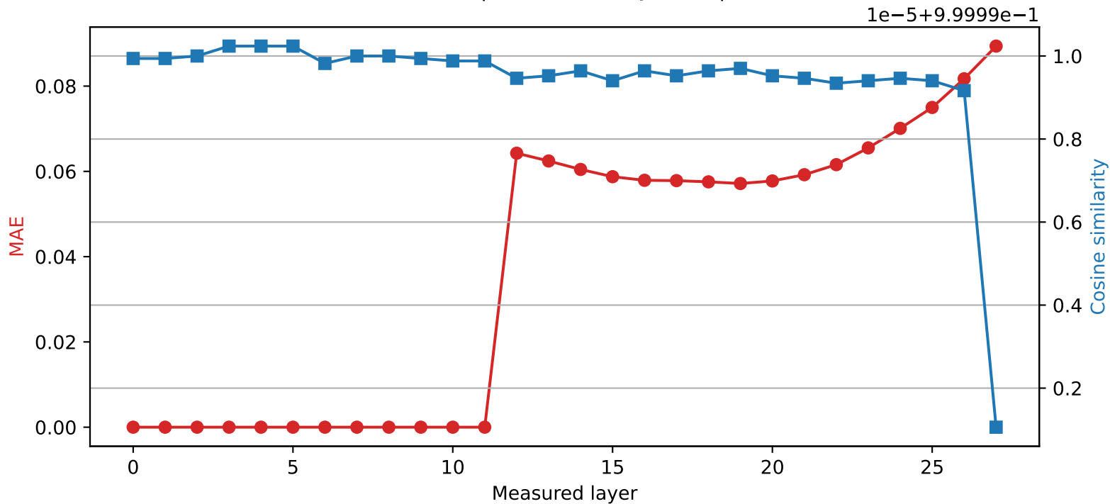
Qwen2.5-7B-Instruct | Quantized layer 11 | float32 \rightarrow int8
