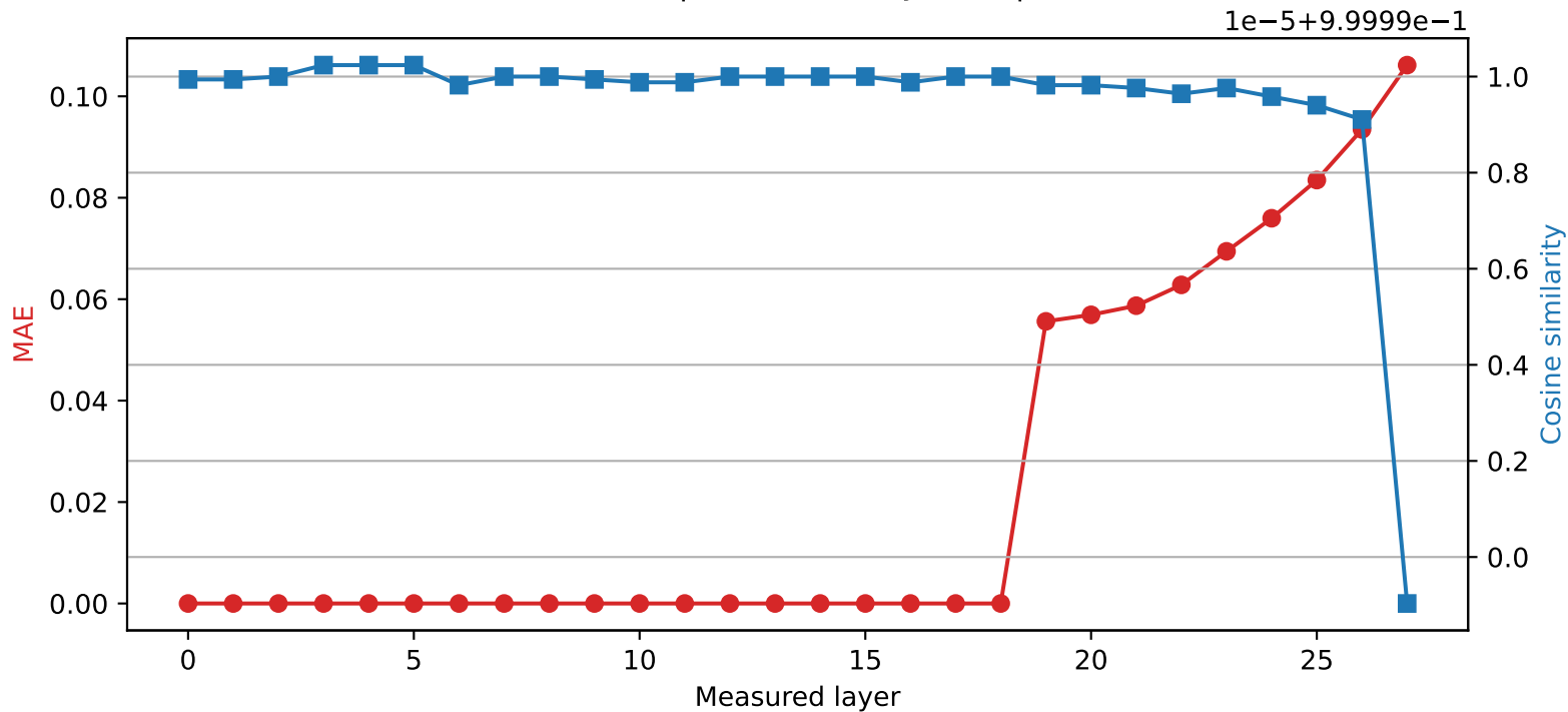
Qwen2.5-7B-Instruct | Quantized layer 18 | float32 → int8
