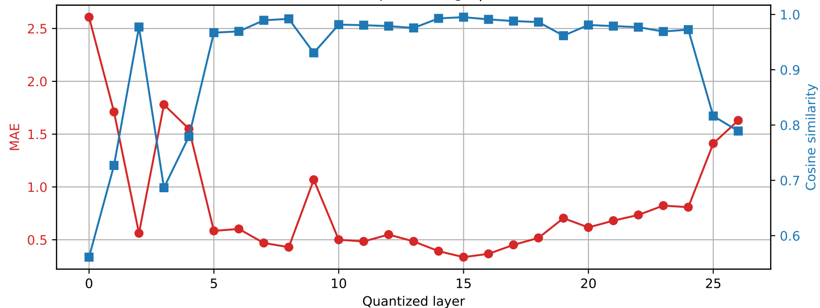
Qwen2.5-7B-Instruct | Prompt 0 Final RMSNorm output damage | float32 \rightarrow int4
