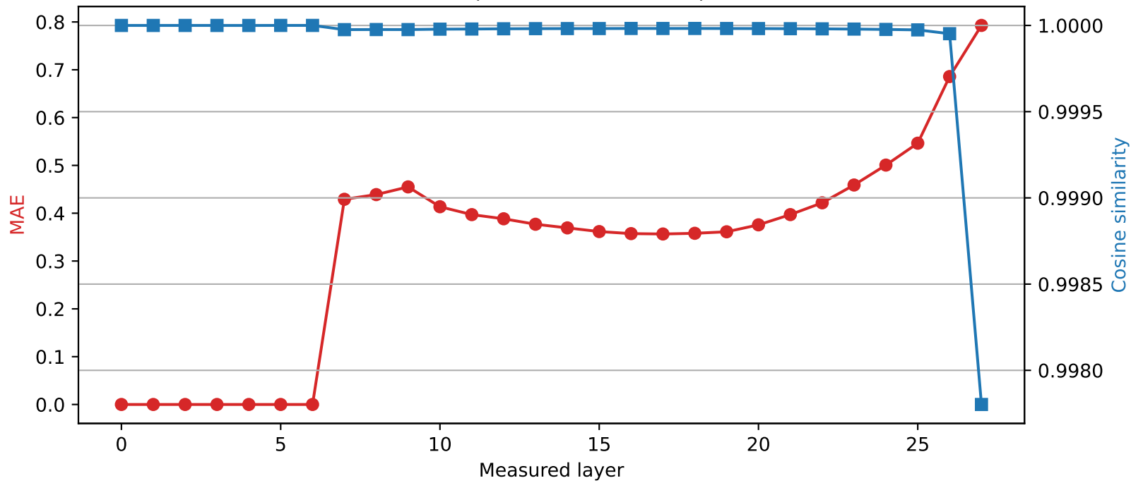
Qwen2.5-7B-Instruct | Quantized layer 6 | float32 \rightarrow int4
