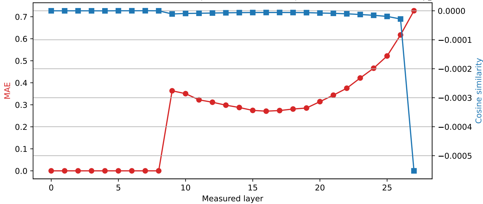
Qwen2.5-7B-Instruct | Quantized layer 8 | float32 → int4
