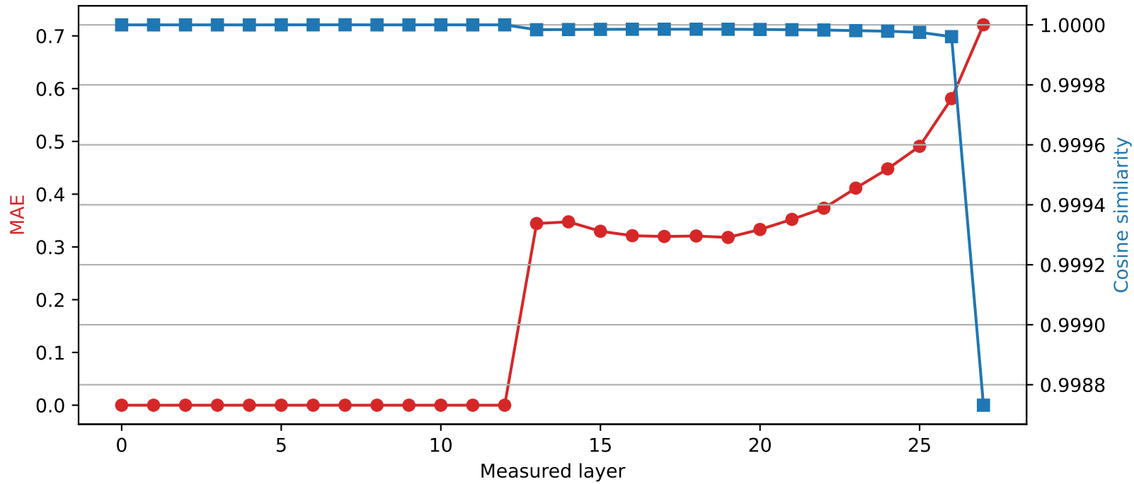
Qwen2.5-7B-Instruct | Quantized layer 12 | float32 \rightarrow int4
