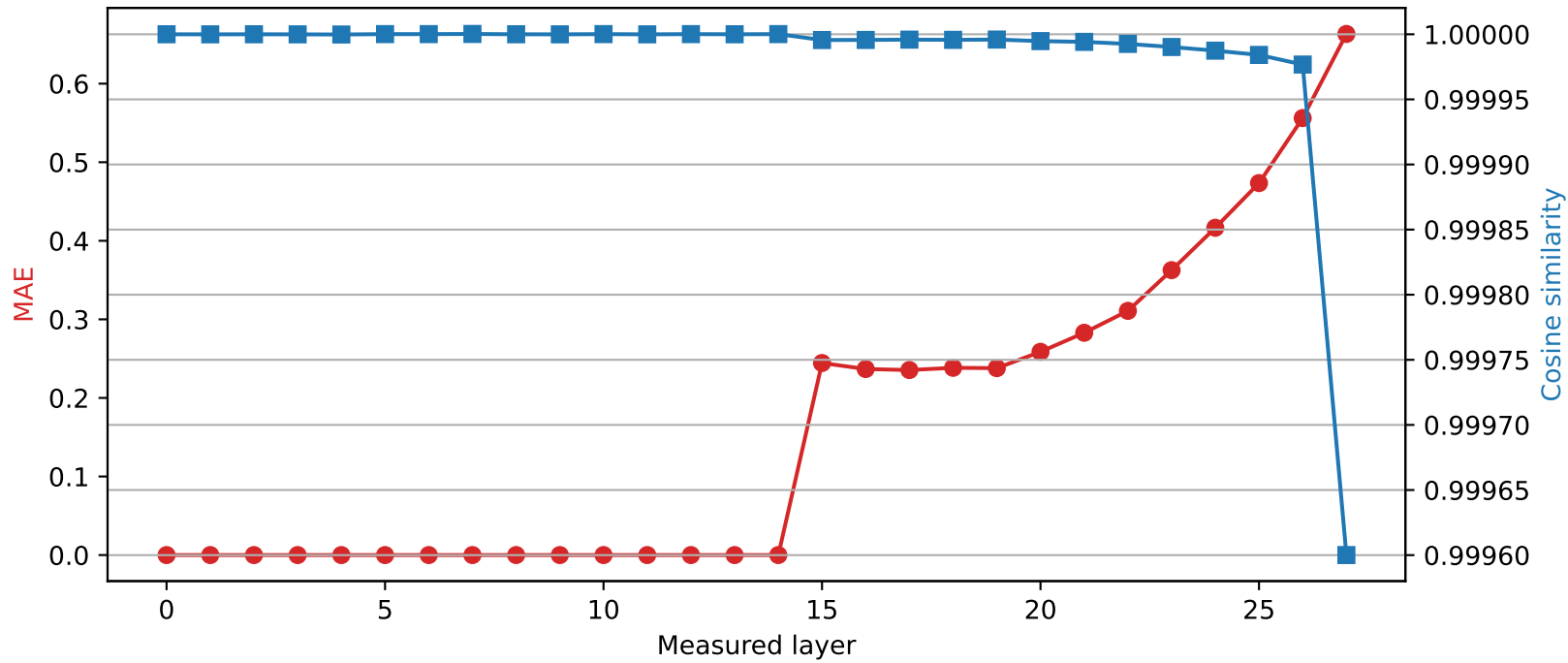
Qwen2.5-7B-Instruct | Quantized layer 14 | float32 \rightarrow int4
