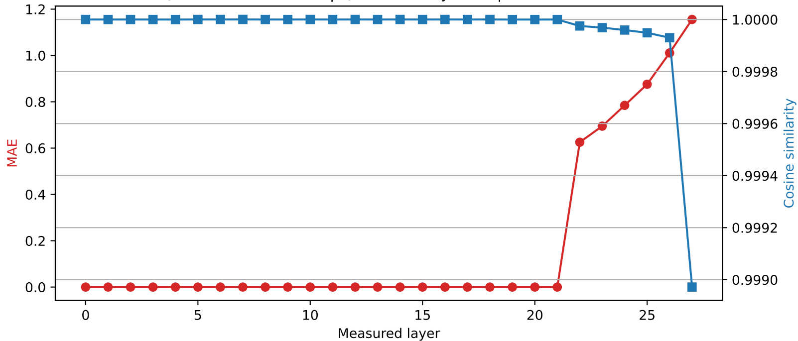
Qwen2.5-7B-Instruct | Quantized layer 21 | float32 \rightarrow int4
