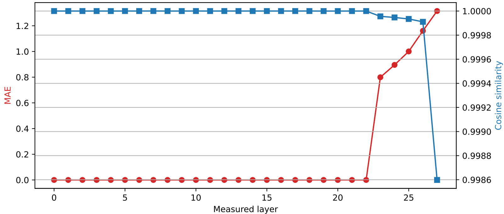
Qwen2.5-7B-Instruct | Quantized layer 22 | float32 \rightarrow int4
