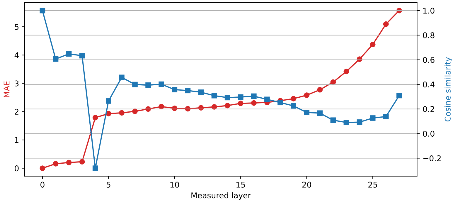
Qwen2.5-7B-Instruct | Quantized layer 0 | float32 \rightarrow int4
