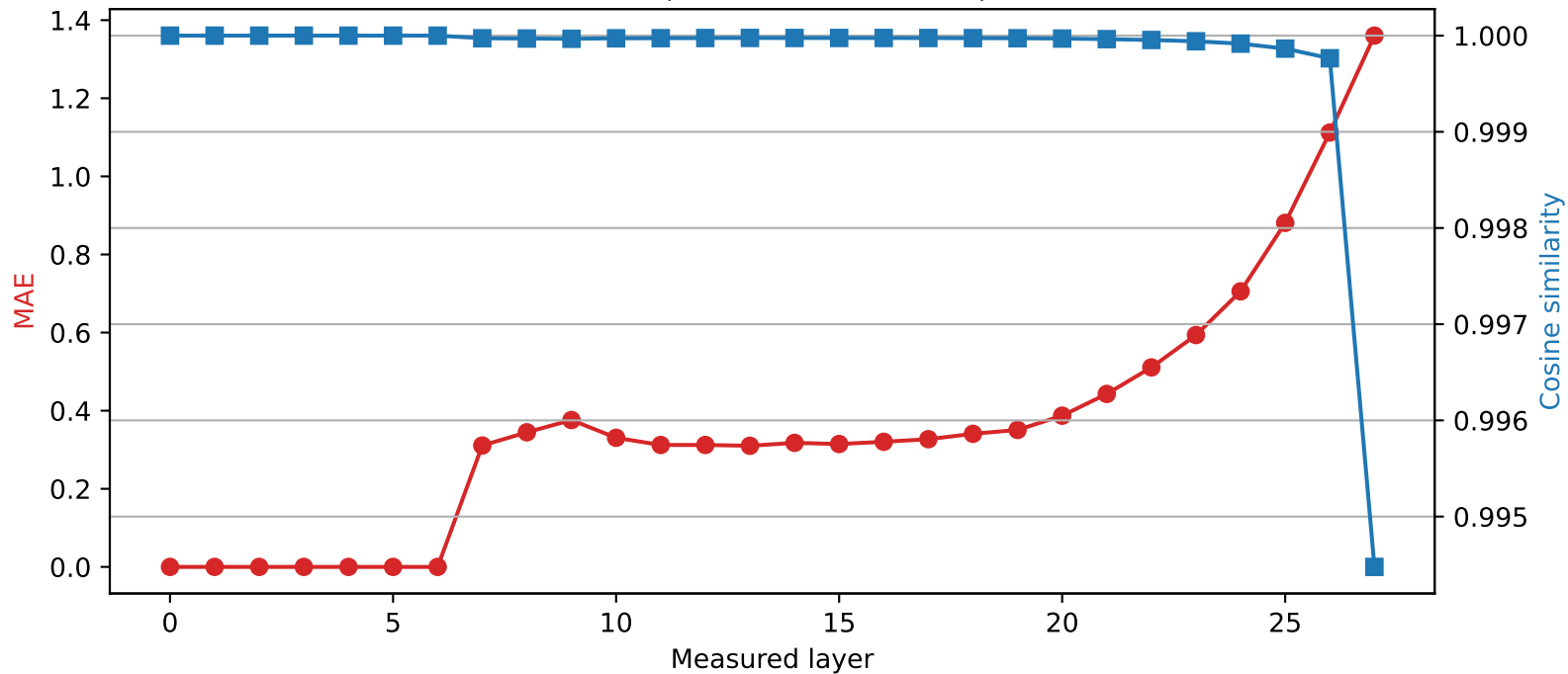
Qwen2.5-7B-Instruct | Quantized layer 6 | float32 → int4
