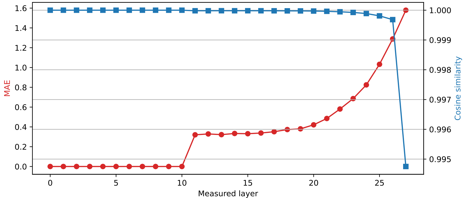
Qwen2.5-7B-Instruct | Quantized layer 10 | float32 \rightarrow int4
