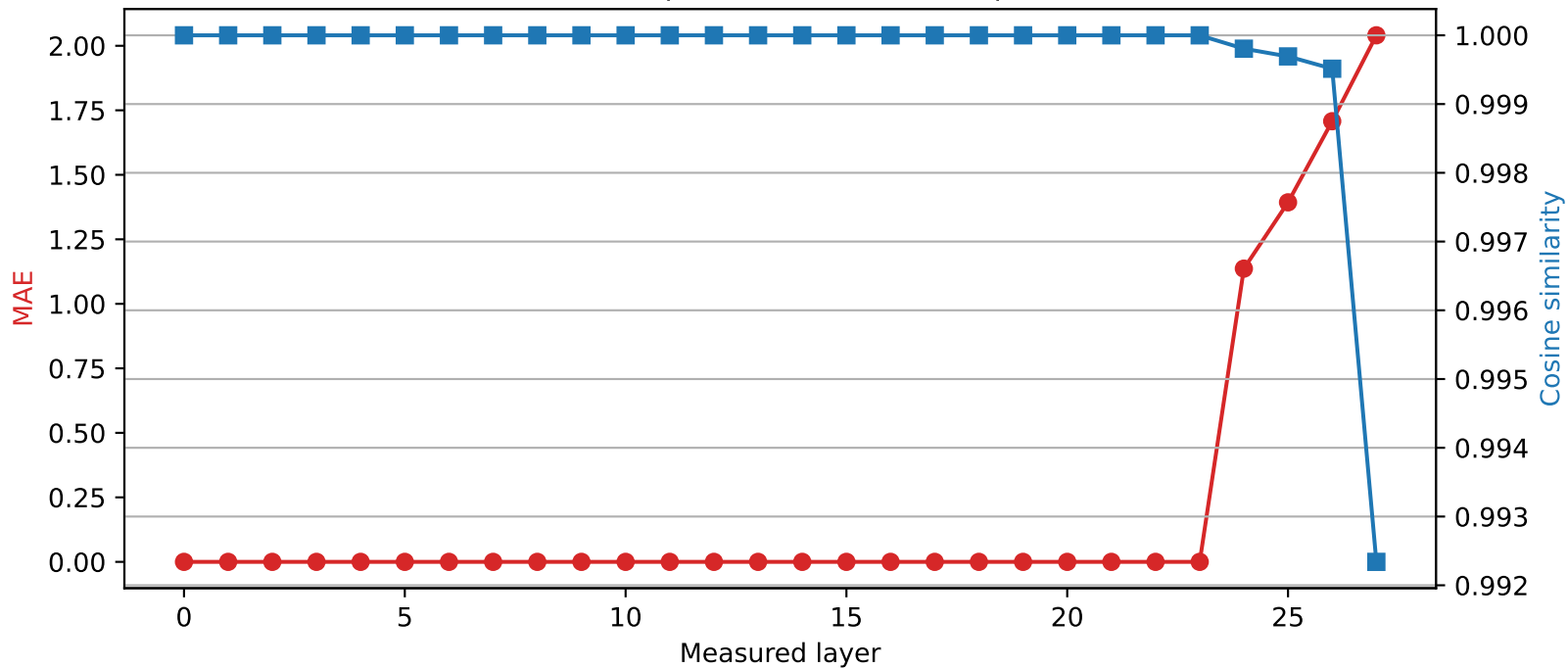
Qwen2.5-7B-Instruct | Quantized layer 23 | float32 \rightarrow int4
