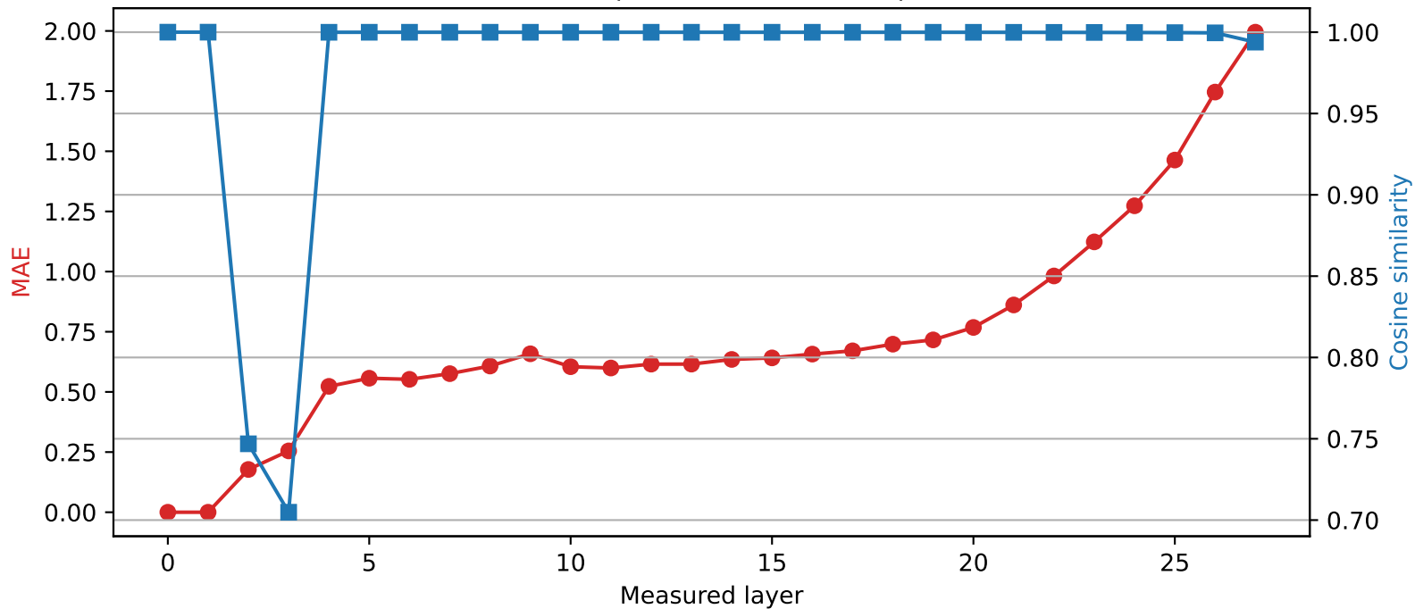
Qwen2.5-7B-Instruct | Quantized layer 1 | float32 \rightarrow int4
