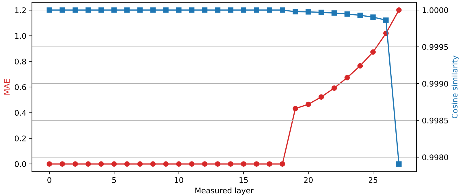
Qwen2.5-7B-Instruct | Quantized layer 18 | float32 \rightarrow int4
