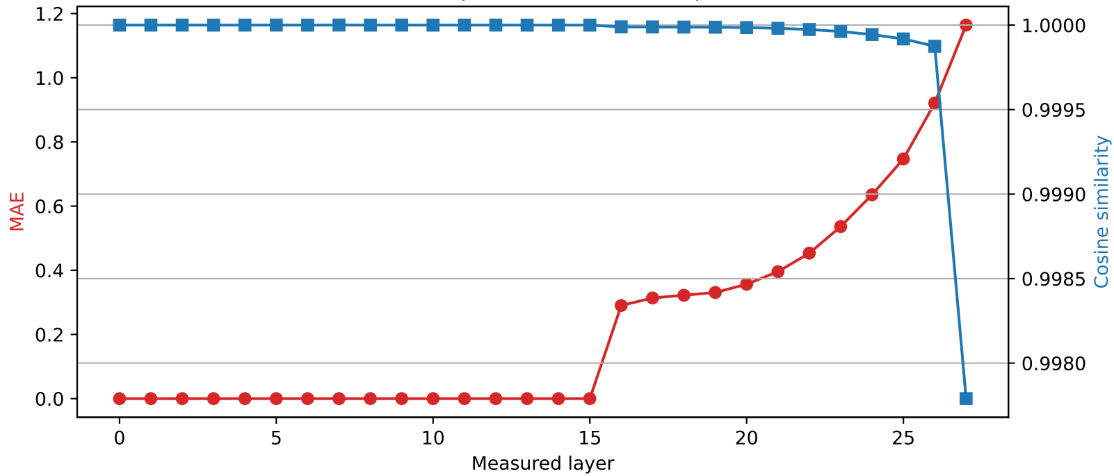
Qwen2.5-7B-Instruct | Quantized layer 15 | float32 \rightarrow int4
