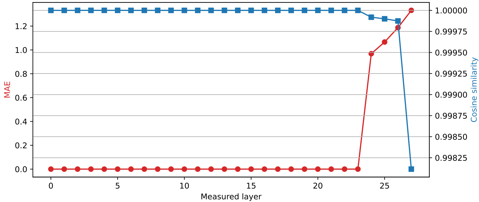
Qwen2.5-7B-Instruct | Quantized layer 23 | float32 → int4
