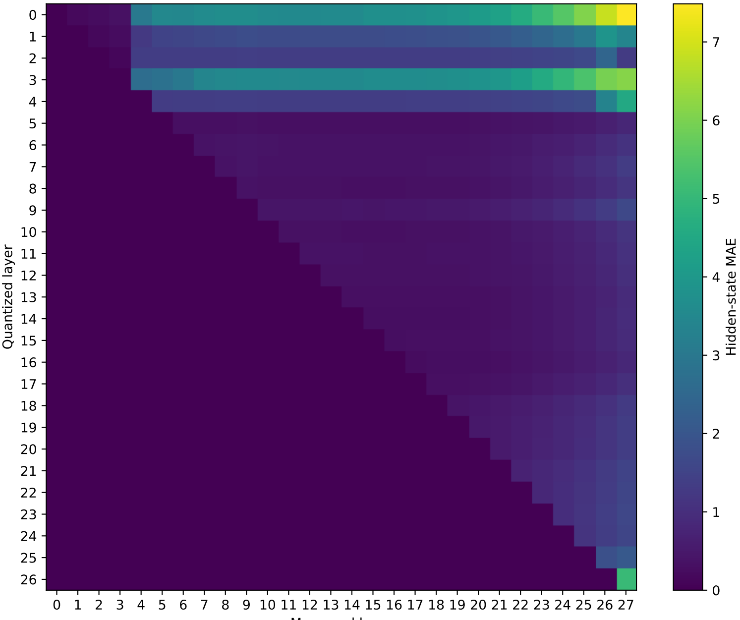
Model: Qwen2.5-7B-Instruct | float32 \rightarrow int2
