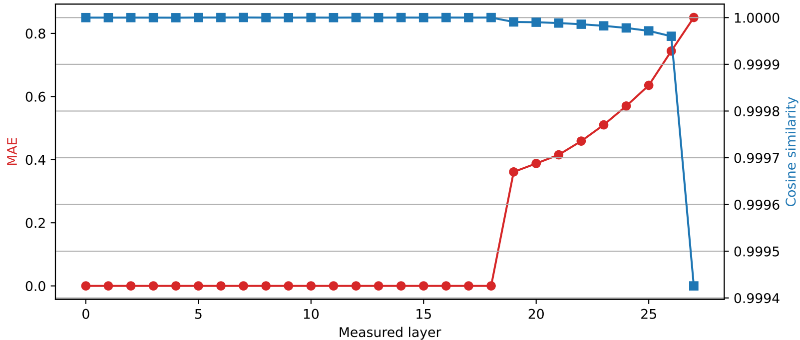
Qwen2.5-7B-Instruct | Quantized layer 18 | float32 \rightarrow int2
