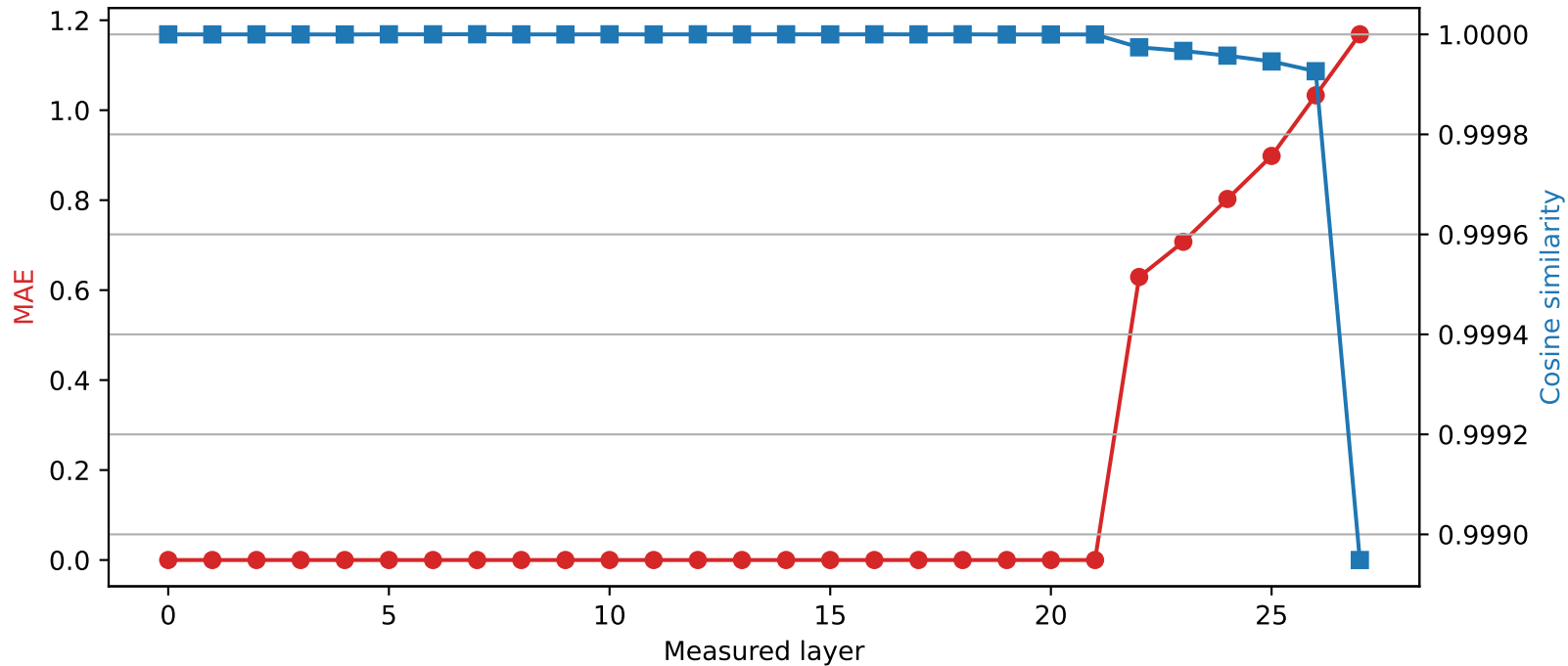
Qwen2.5-7B-Instruct | Quantized layer 21 | float32 \rightarrow int2
