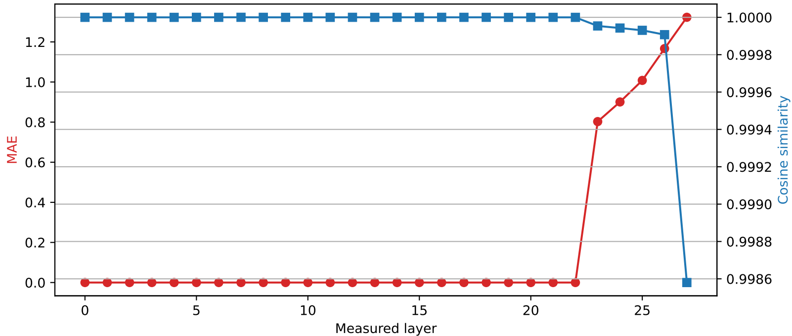
Qwen2.5-7B-Instruct | Quantized layer 22 | float32 \rightarrow int2
