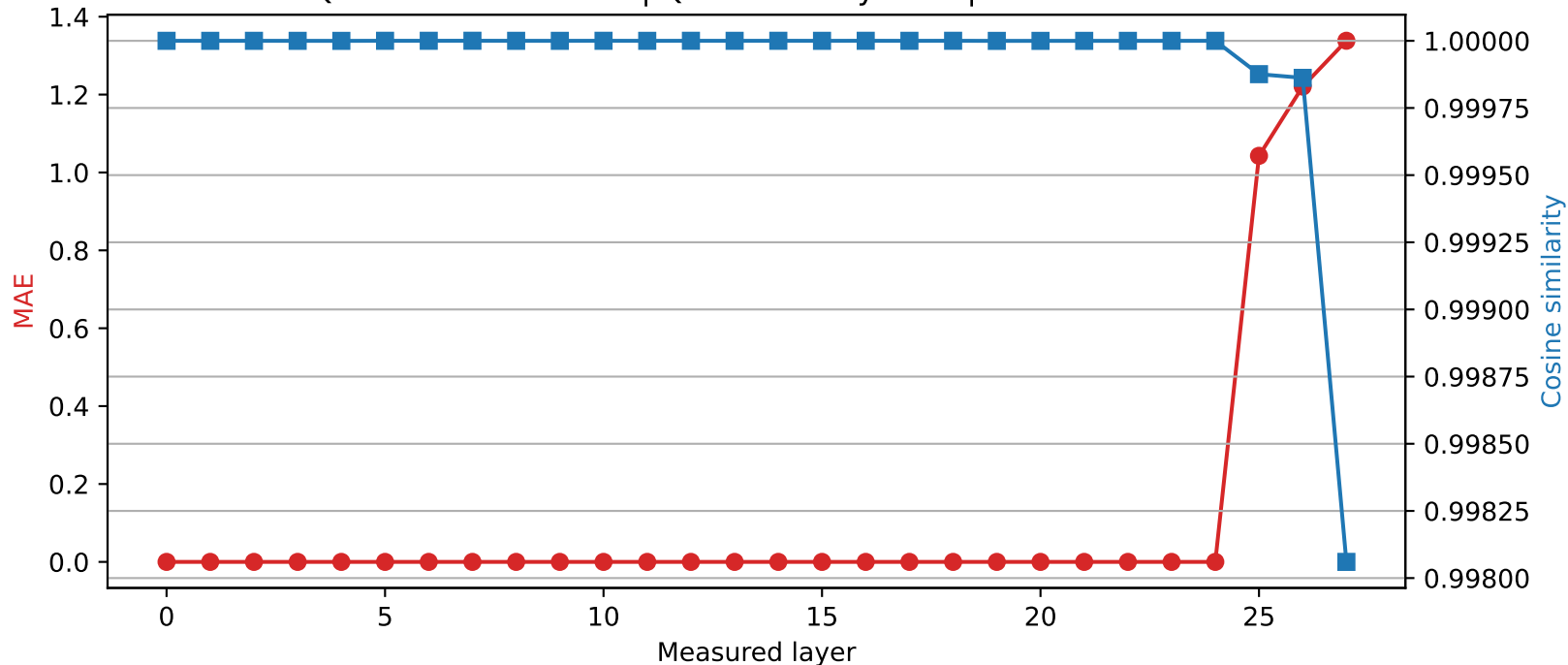
Qwen2.5-7B-Instruct | Quantized layer 24 | float32 \rightarrow int2
