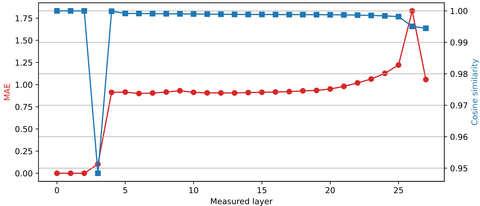
Qwen2.5-7B-Instruct | Quantized layer 2 | float32 → int2
