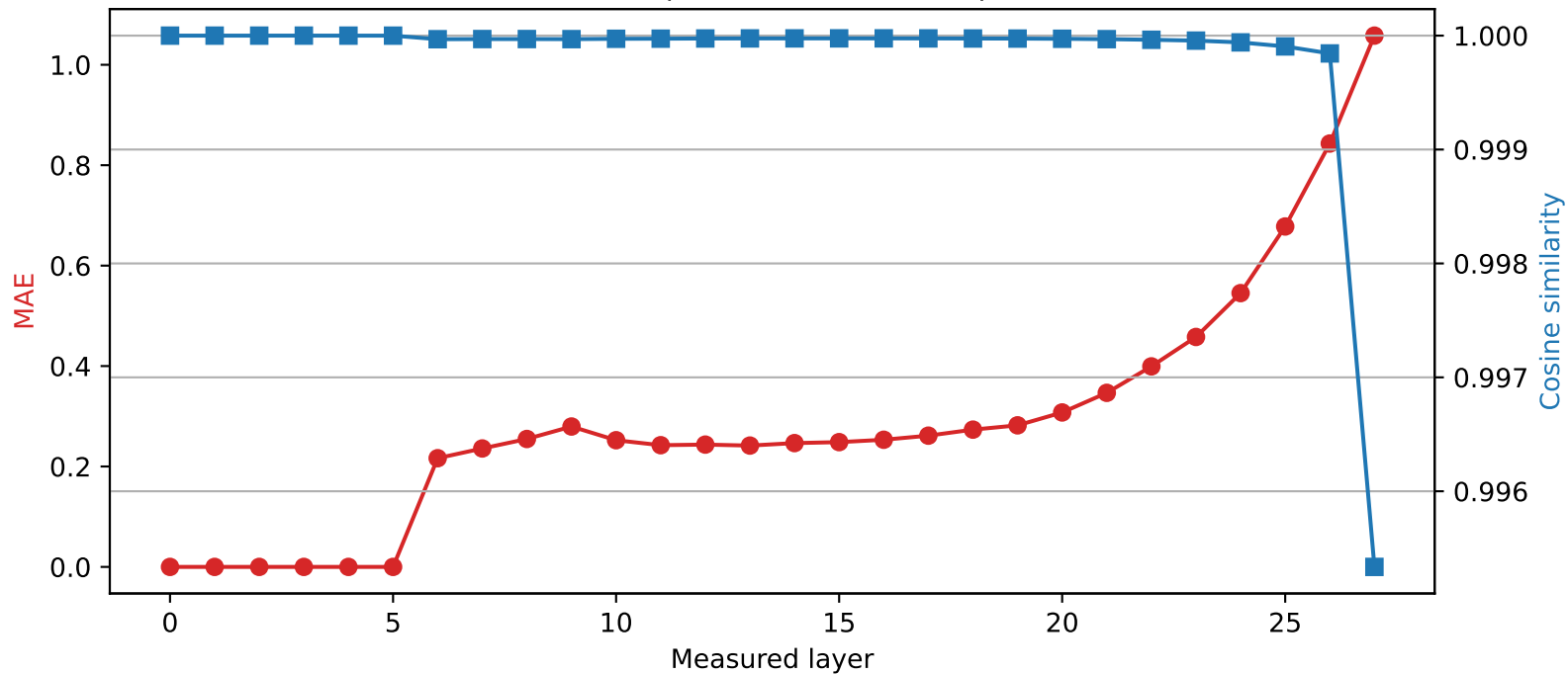
Qwen2.5-7B-Instruct | Quantized layer 5 | float32 \rightarrow int2
