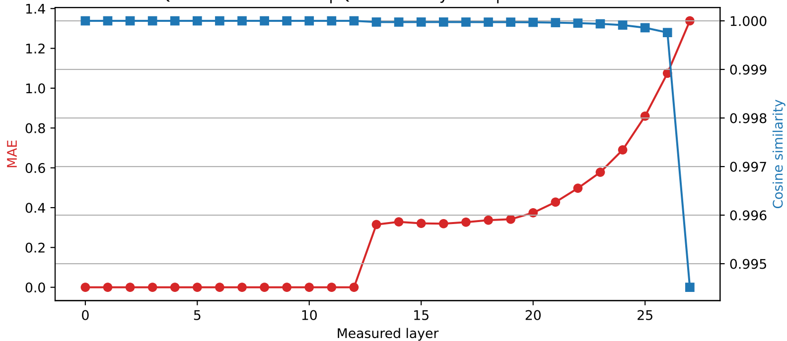
Qwen2.5-7B-Instruct | Quantized layer 12 | float32 \rightarrow int2
