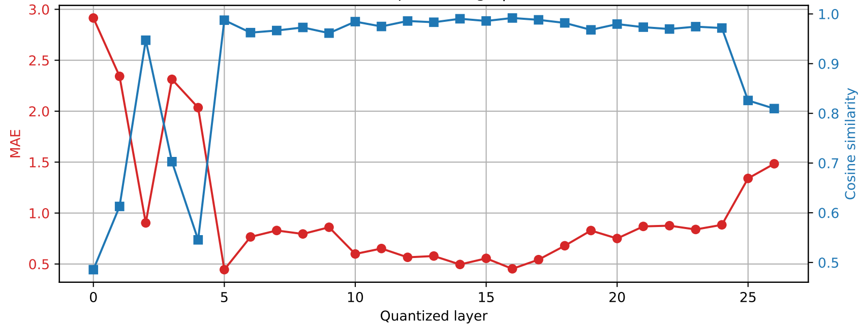
Qwen2.5-7B-Instruct | Prompt 2 Final RMSNorm output damage | float32 \rightarrow int2
