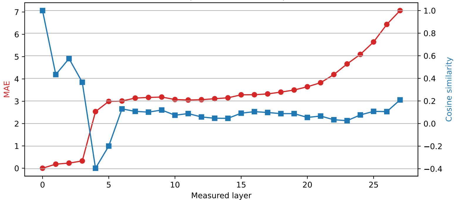
Qwen2.5-7B-Instruct | Quantized layer 0 | float32 \rightarrow int2
