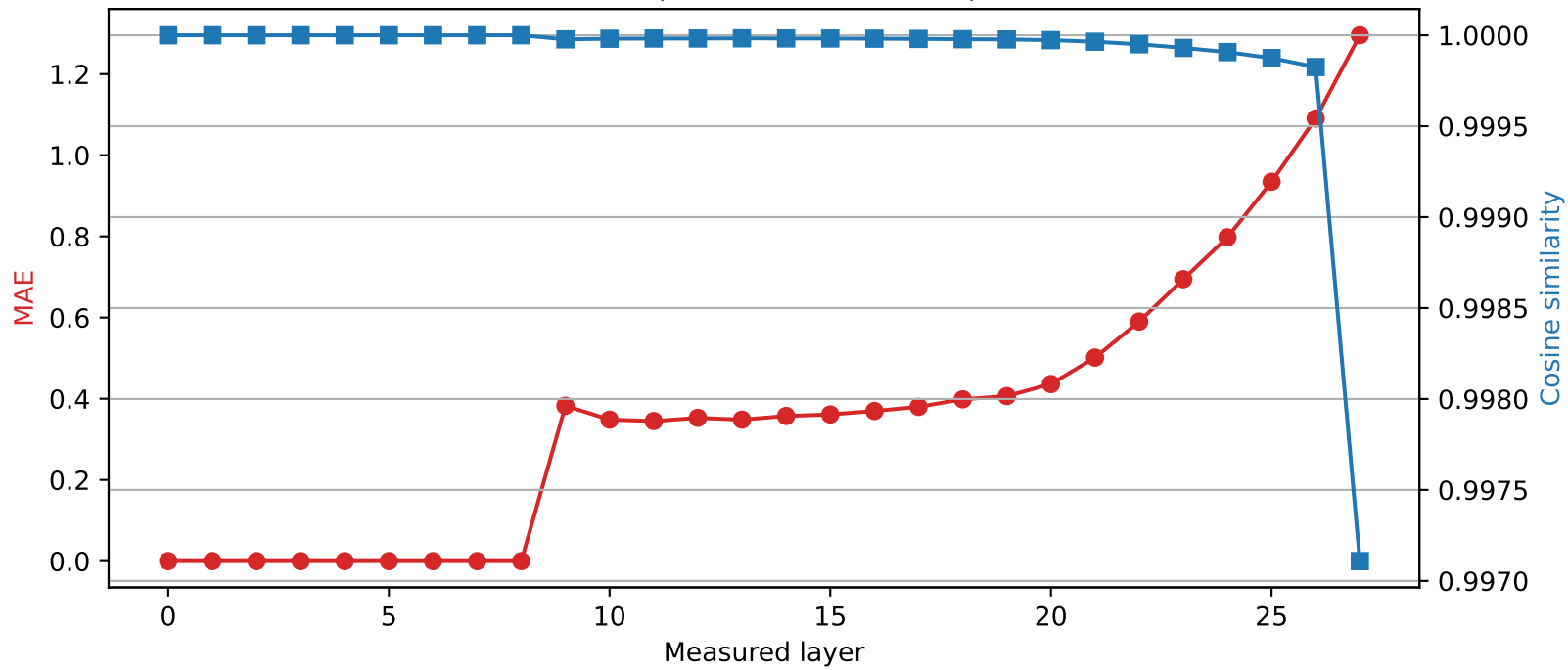
Qwen2.5-7B-Instruct | Quantized layer 8 | float32 → int2
