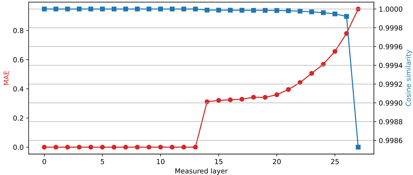
Qwen2.5-7B-Instruct | Quantized layer 13 | float32 \rightarrow int2
