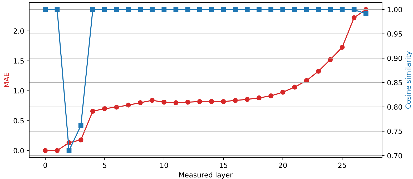
Qwen2.5-7B-Instruct | Quantized layer 1 | float32 \rightarrow int2
