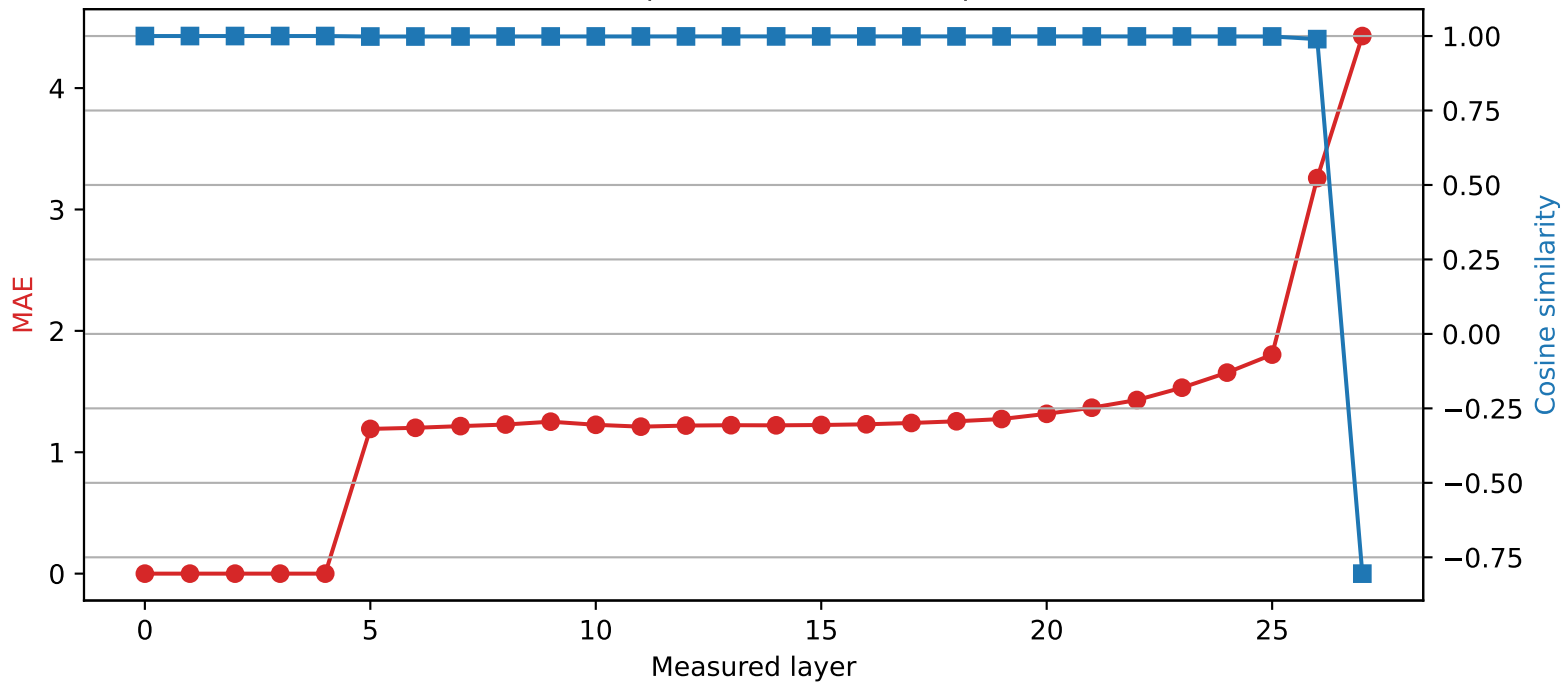
Qwen2.5-7B-Instruct | Quantized layer 4 | float32 → int2
