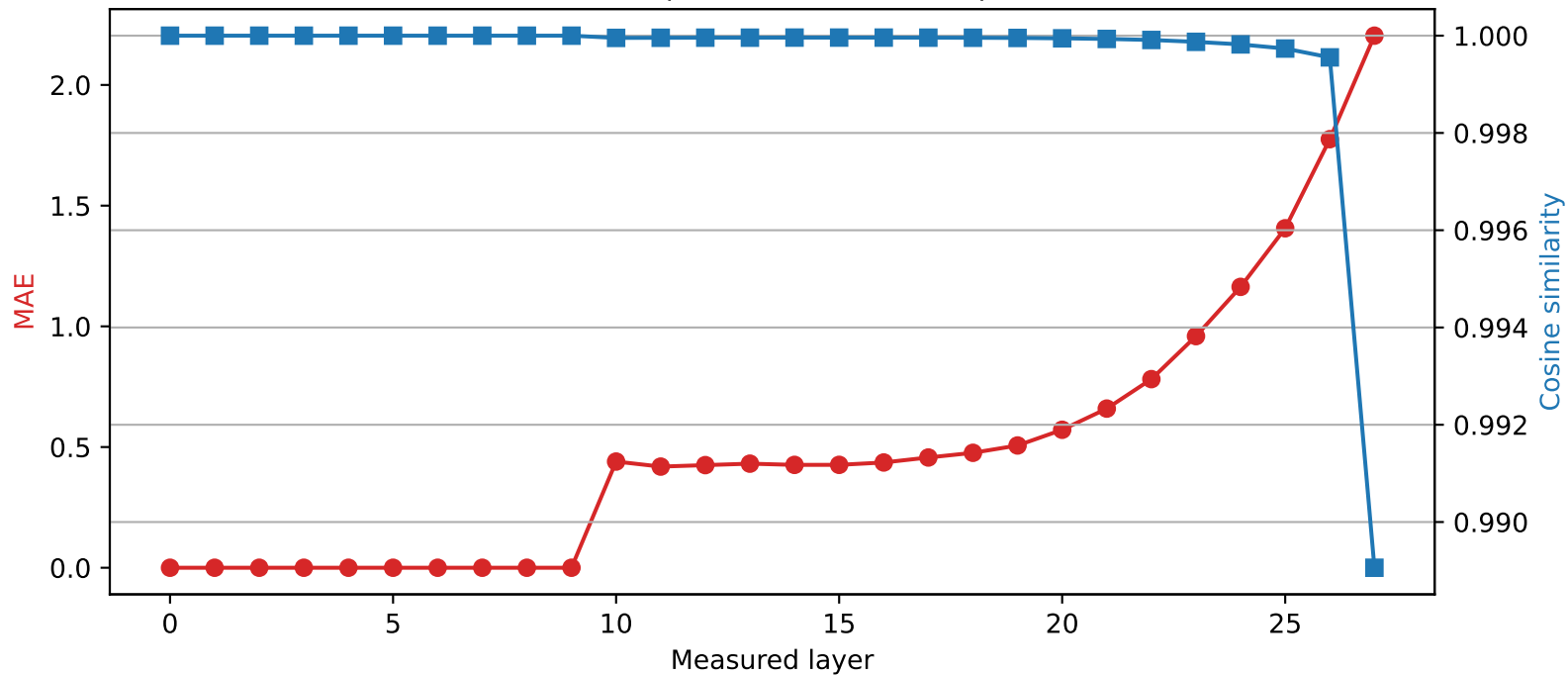
Qwen2.5-7B-Instruct | Quantized layer 9 | float32 \rightarrow int2
