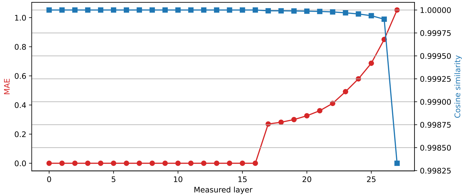
Qwen2.5-7B-Instruct | Quantized layer 16 | float32 \rightarrow int2
