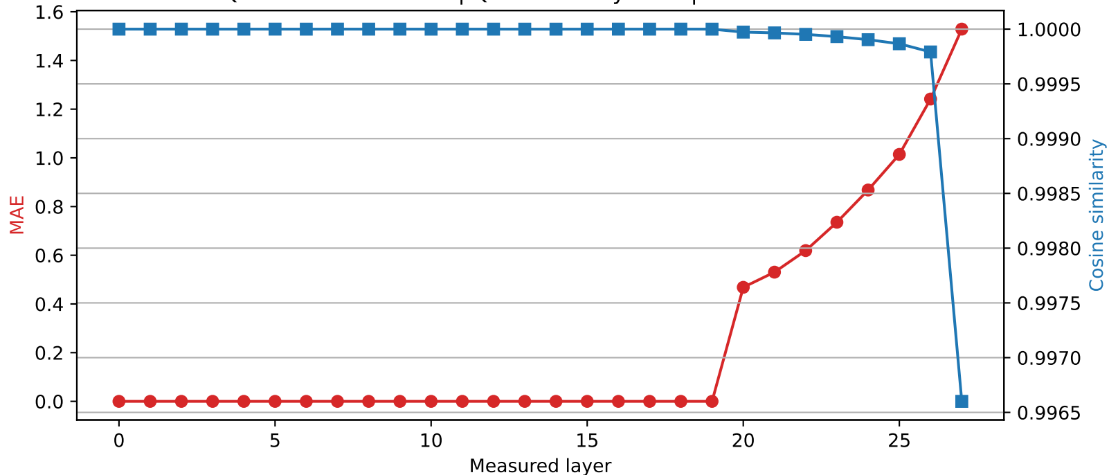
Qwen2.5-7B-Instruct | Quantized layer 19 | float32 → int2
