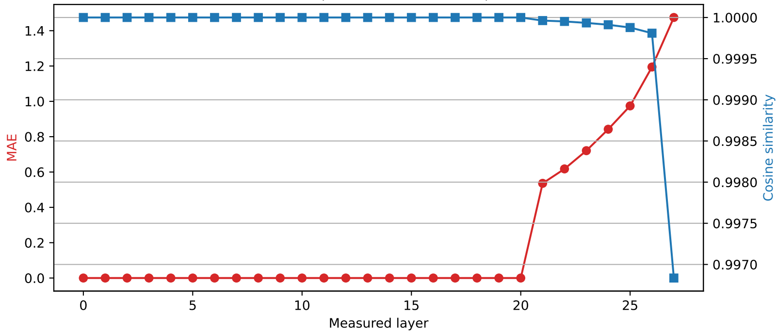
Qwen2.5-7B-Instruct | Quantized layer 20 | float32 → int2
