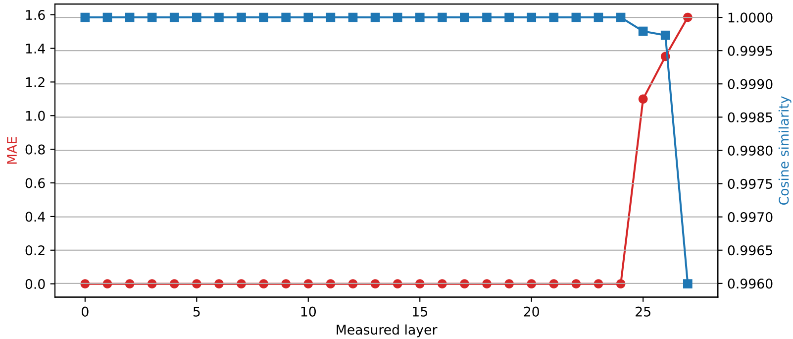
Qwen2.5-7B-Instruct | Quantized layer 24 | float32 → int2
