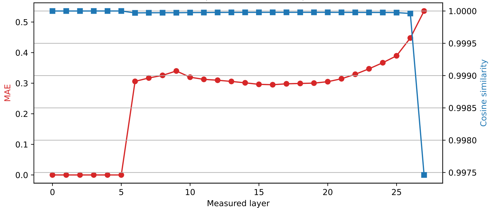
Qwen2.5-7B-Instruct | Quantized layer 5 | float32 → int2
