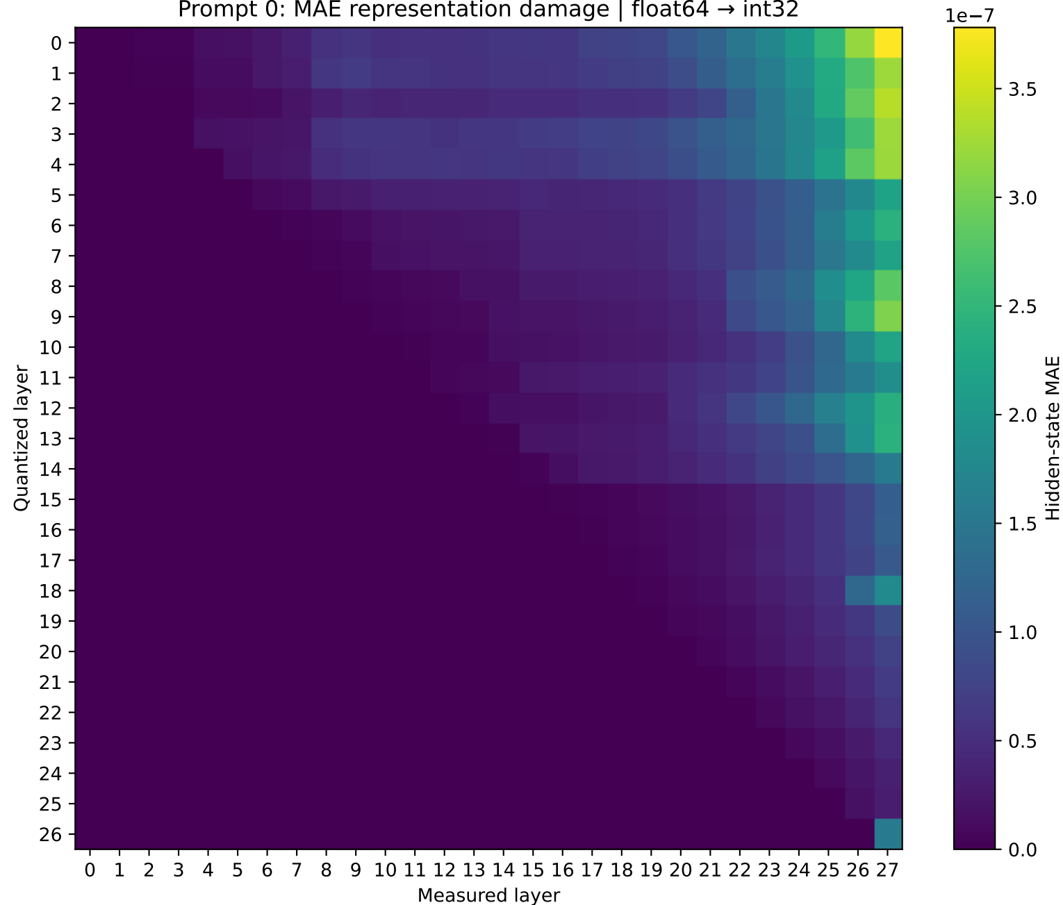
Qwen2.5-7B-Instruct Prompt 0: MAE representation damage | float64 → int32
