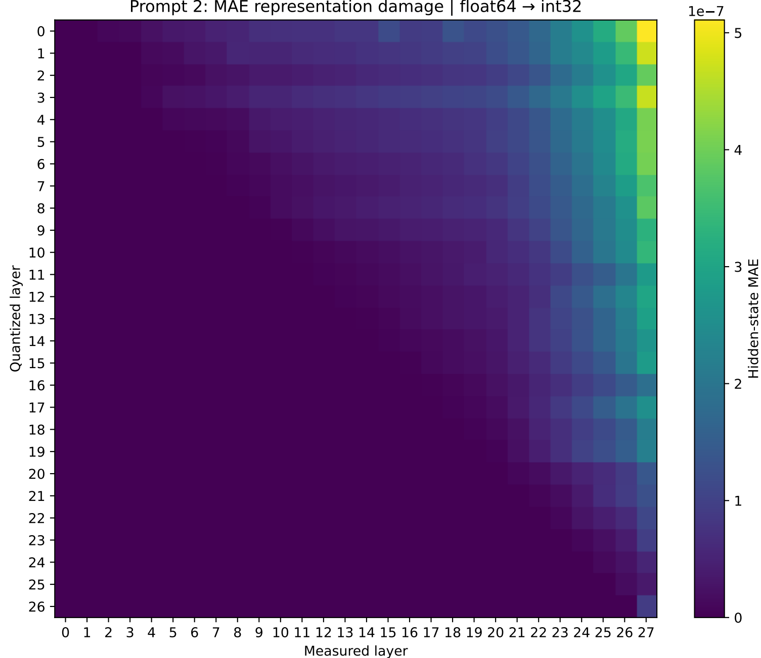
Prompt 2: MAE representation damage | float64 → int32
