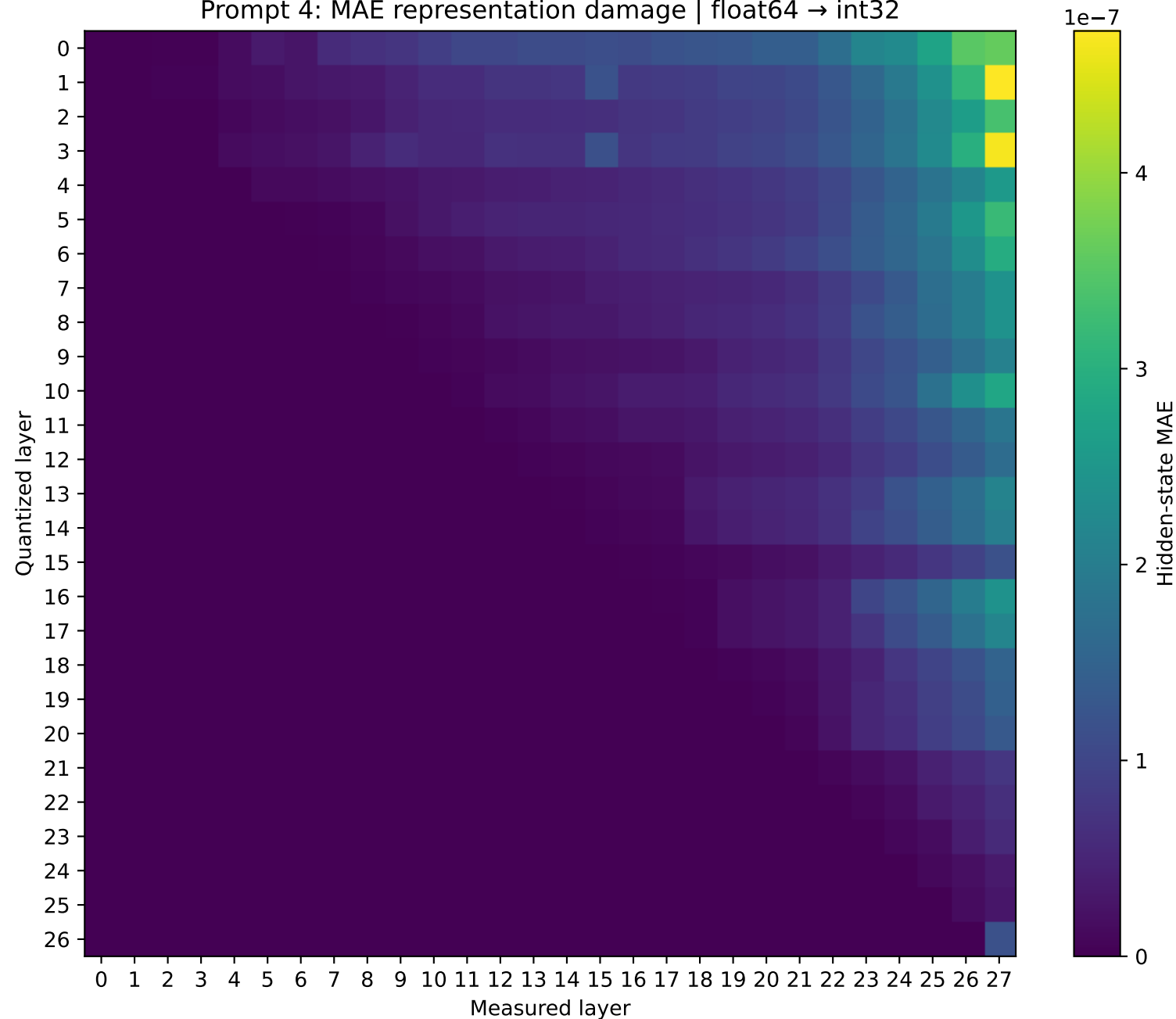
Qwen2.5-7B-Instruct Prompt 4: MAE representation damage | float64 → int32
