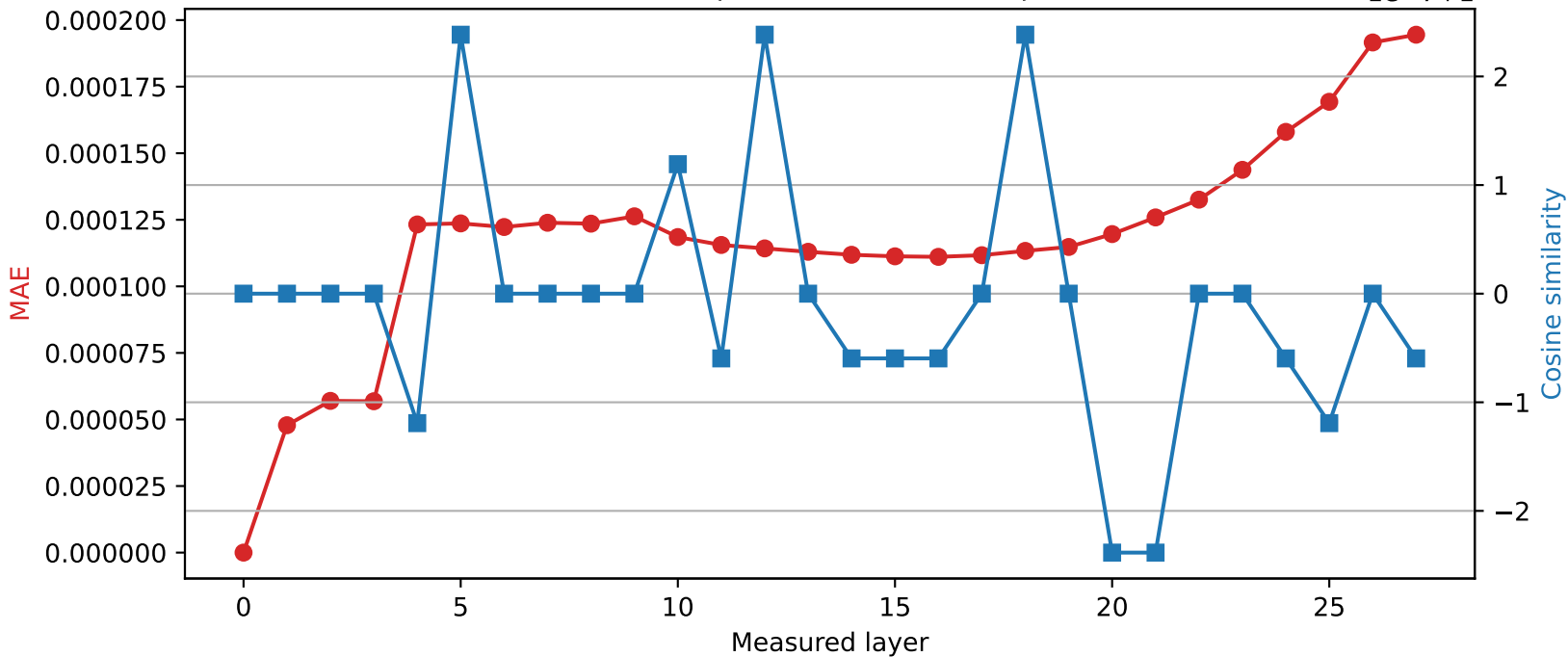
Qwen2.5-7B-Instruct | Quantized layer 0 | float64 → int16
